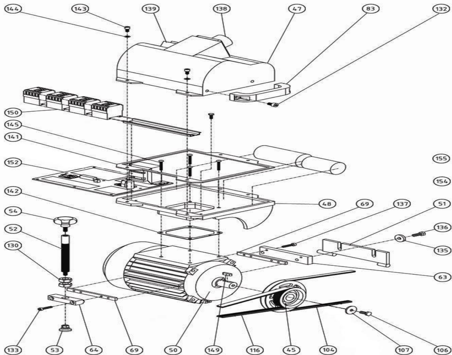
Bona Belt Previous Models AMO110018.3 Belt Motor
