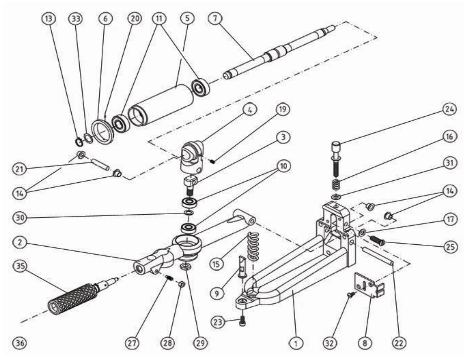
Bona Belt Previous Models AMO110018.3 Belt Tension device
