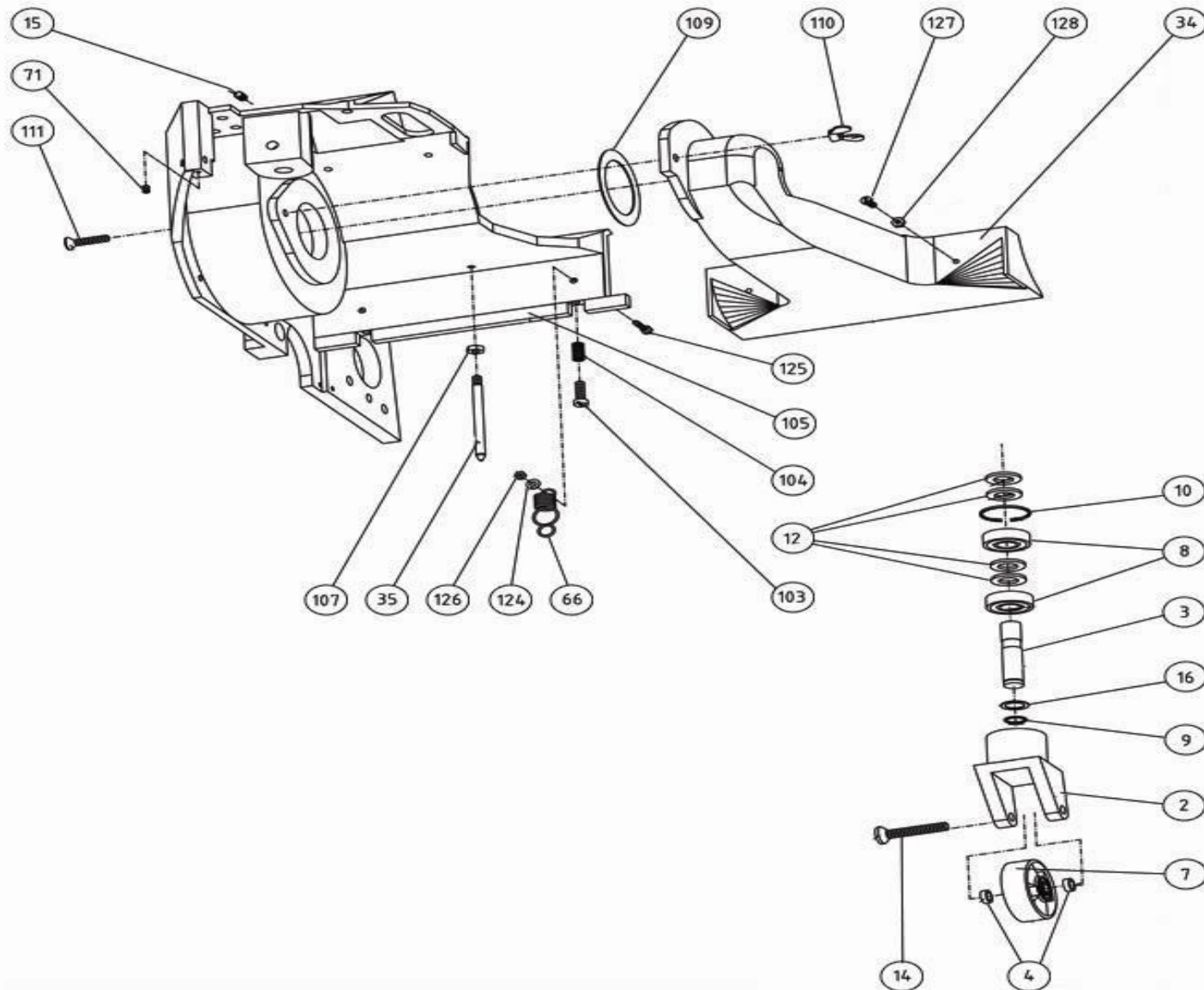
Bona Belt Previous Models AMO110016.3 Belt rear wheel
