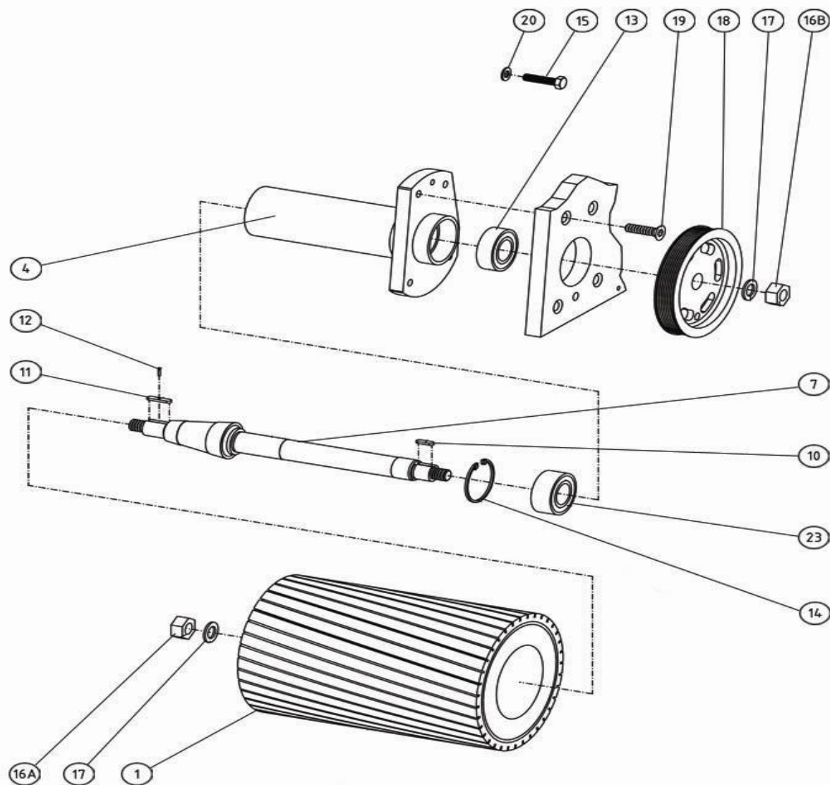
Bona Belt Previous Models AMO110016.3 Belt sanding drum
