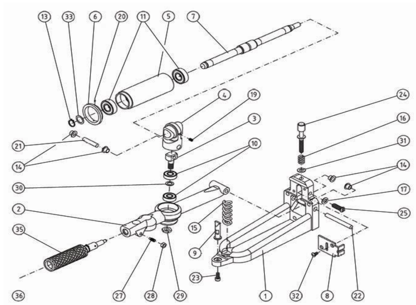
Bona Belt Previous Models AMO110016.3 Belt Tension device
