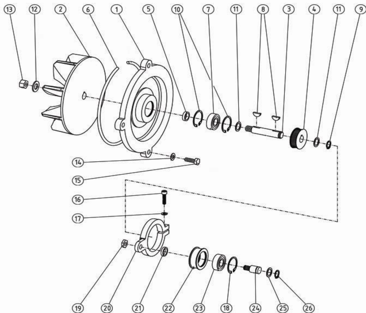
Bona Belt Previous Models AMO110016.3 Belt vacuum cleaner
