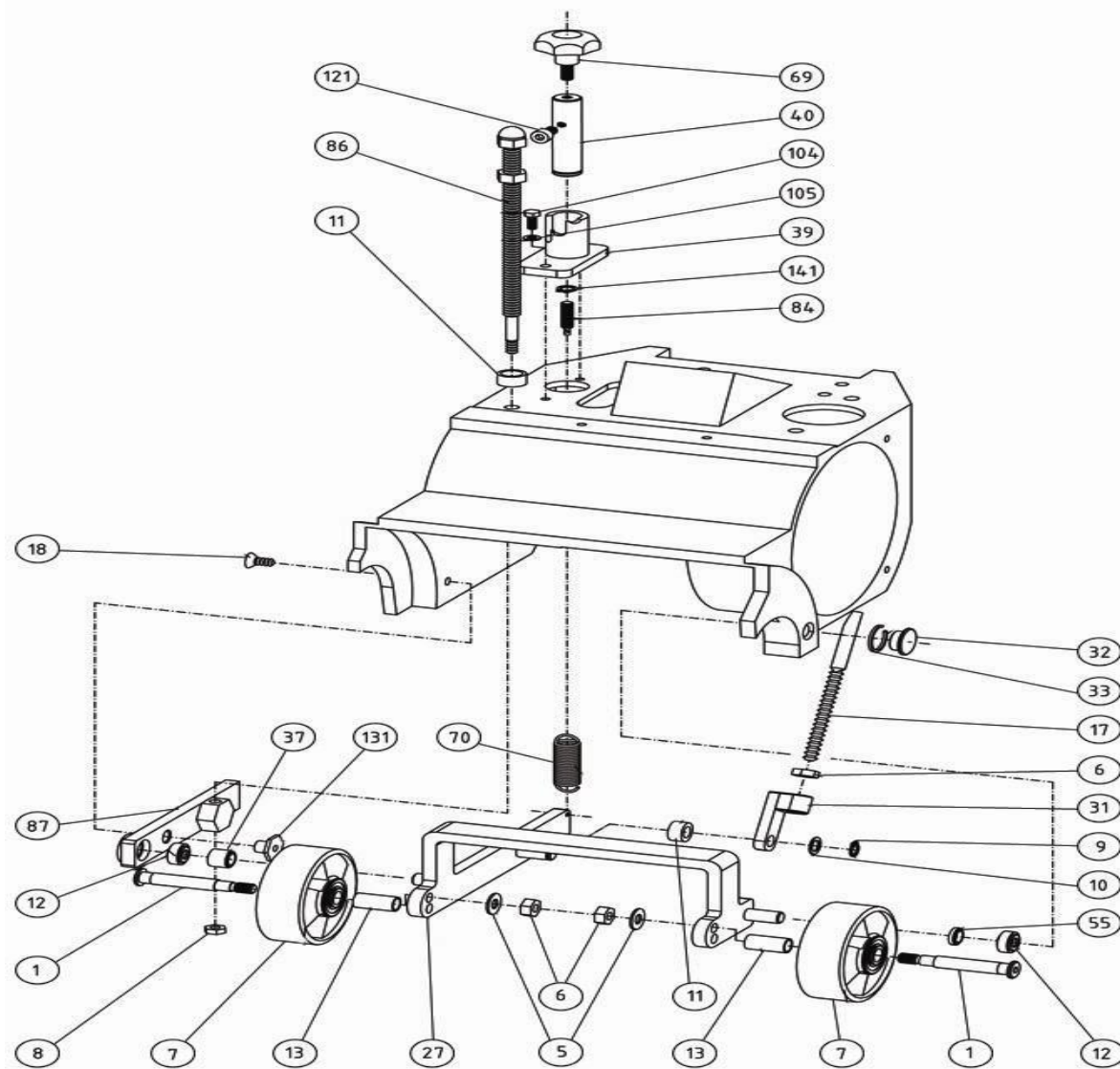
Bona Belt Previous Models AMO110016.3 Belt wheel subframe
