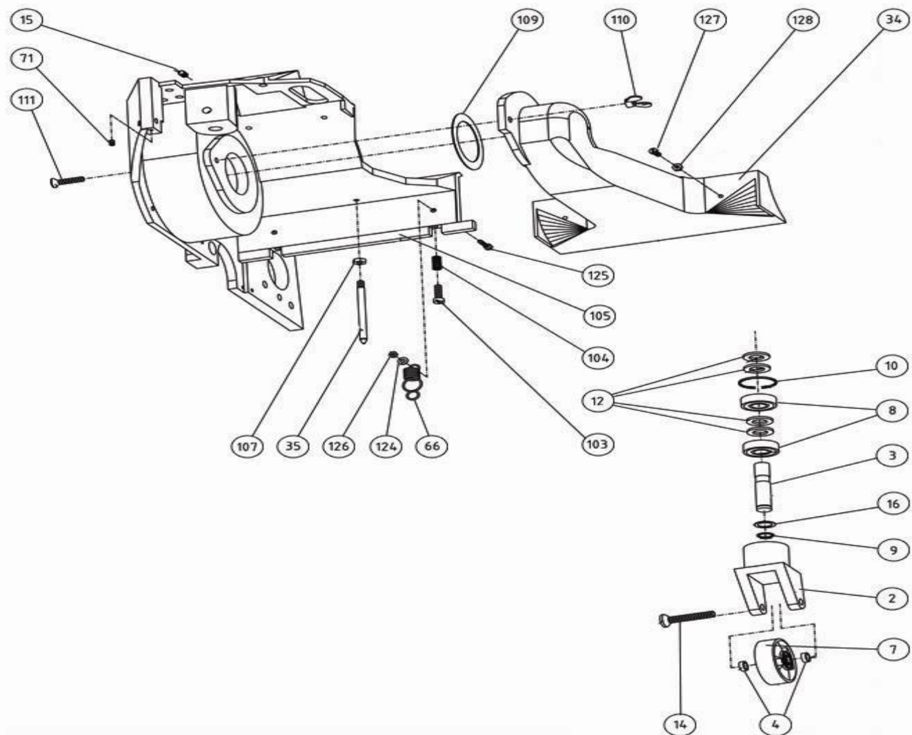
Bona Belt Previous Models AMO110017.3 Belt Rear Wheel
