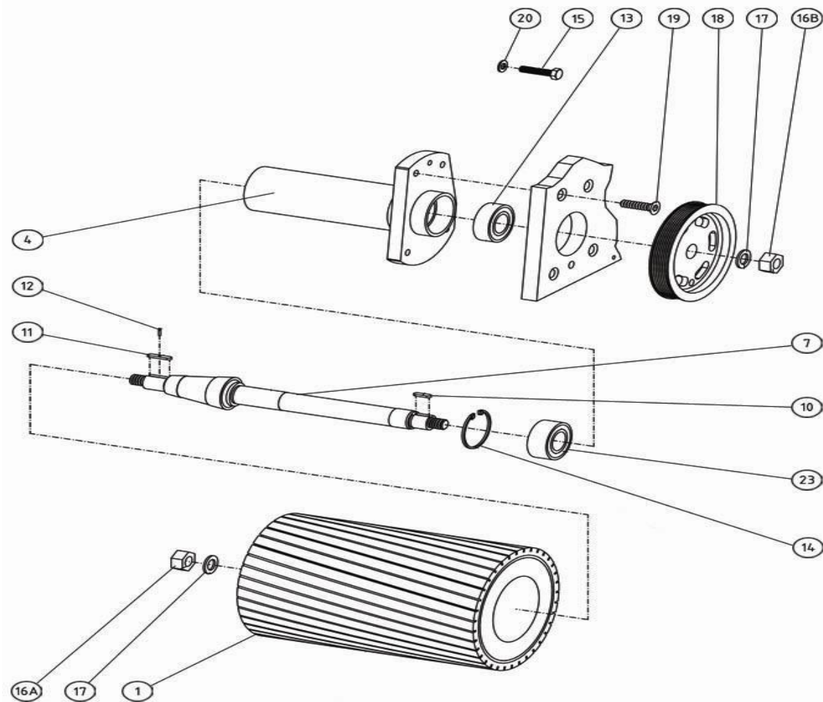
Bona Belt Previous Models AMO110017.3 Belt sanding drum
