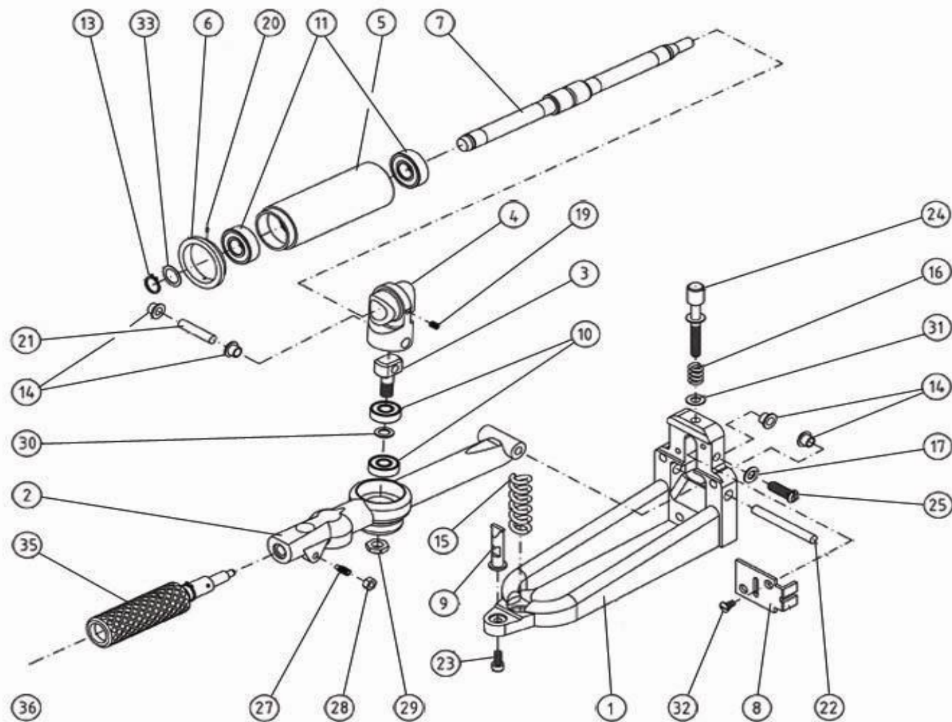
Bona Belt Previous Models AMO110017.3 Belt Tension device
