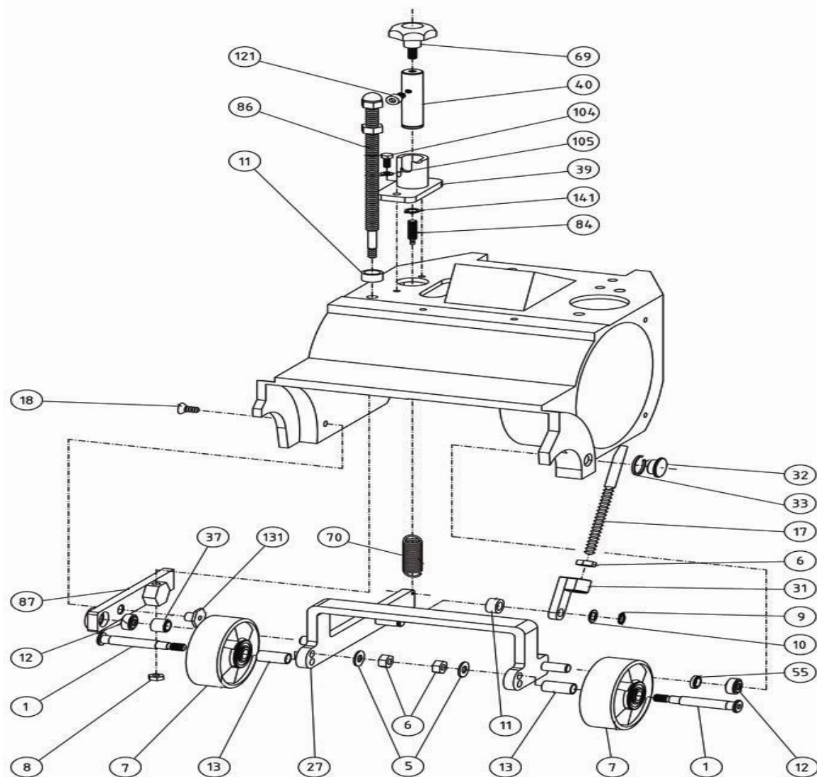
Bona Belt Previous Models AMO110017.3 Belt wheel subframe
