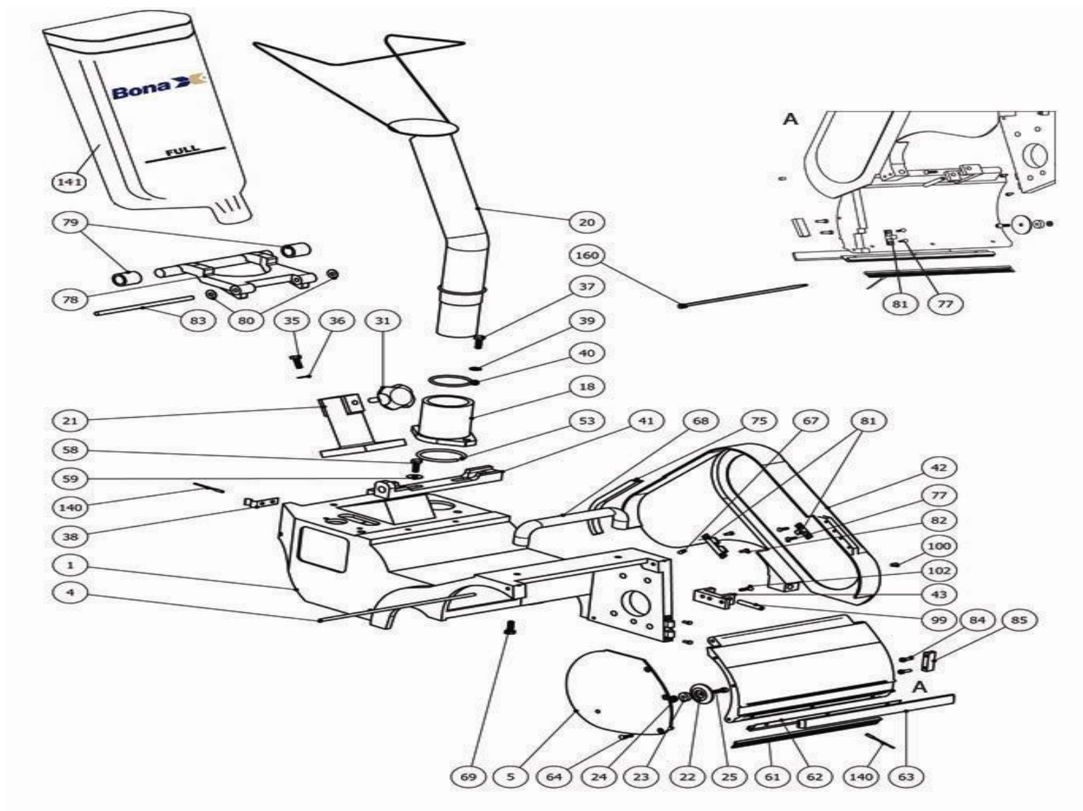
Bona Flexidrum Previous Models AMO150009.2 Flexidrum housing
