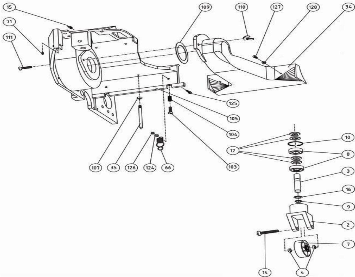
Bona Flexidrum Previous Models AMO150009.2 Flexidrum rear wheel/intake duct compl.
