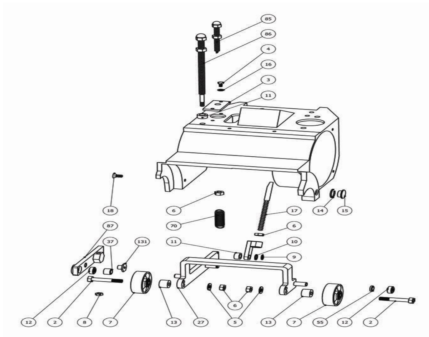
Bona Flexidrum Previous Models AMO150009.2 Flexidrum wheel subframe
