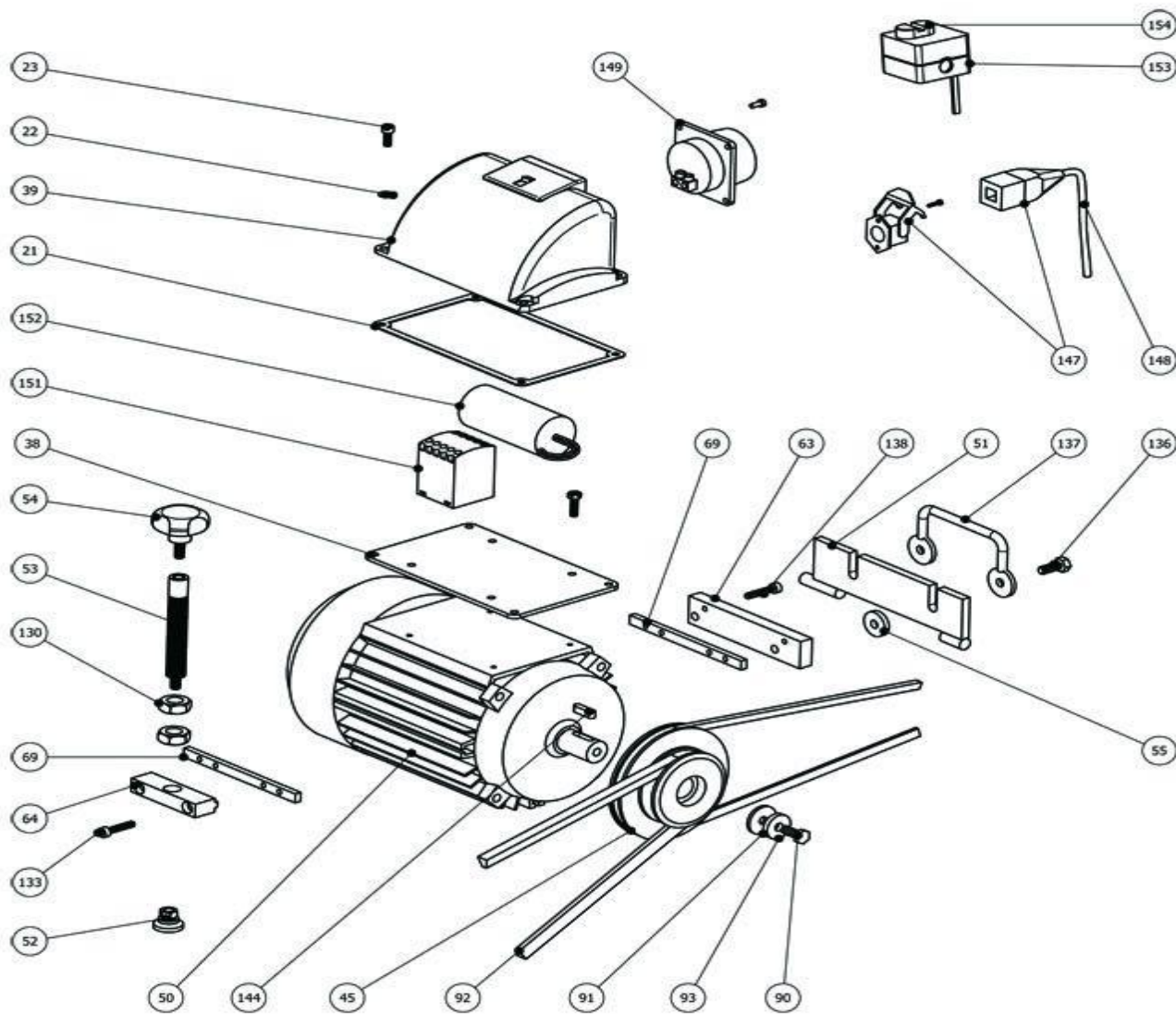
Bona Flexidrum Previous Models AMO150000.2 Flexidrum 1,8 KW Motor
