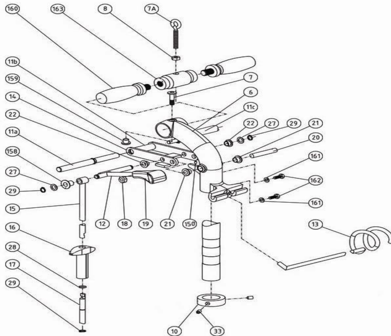
Bona Flexidrum Previous Models AMO150000.2 Flexidrum handle
