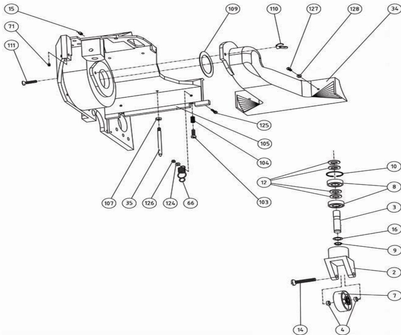
Bona Flexidrum Previous Models AMO150000.2 Flexidrum rear wheel
