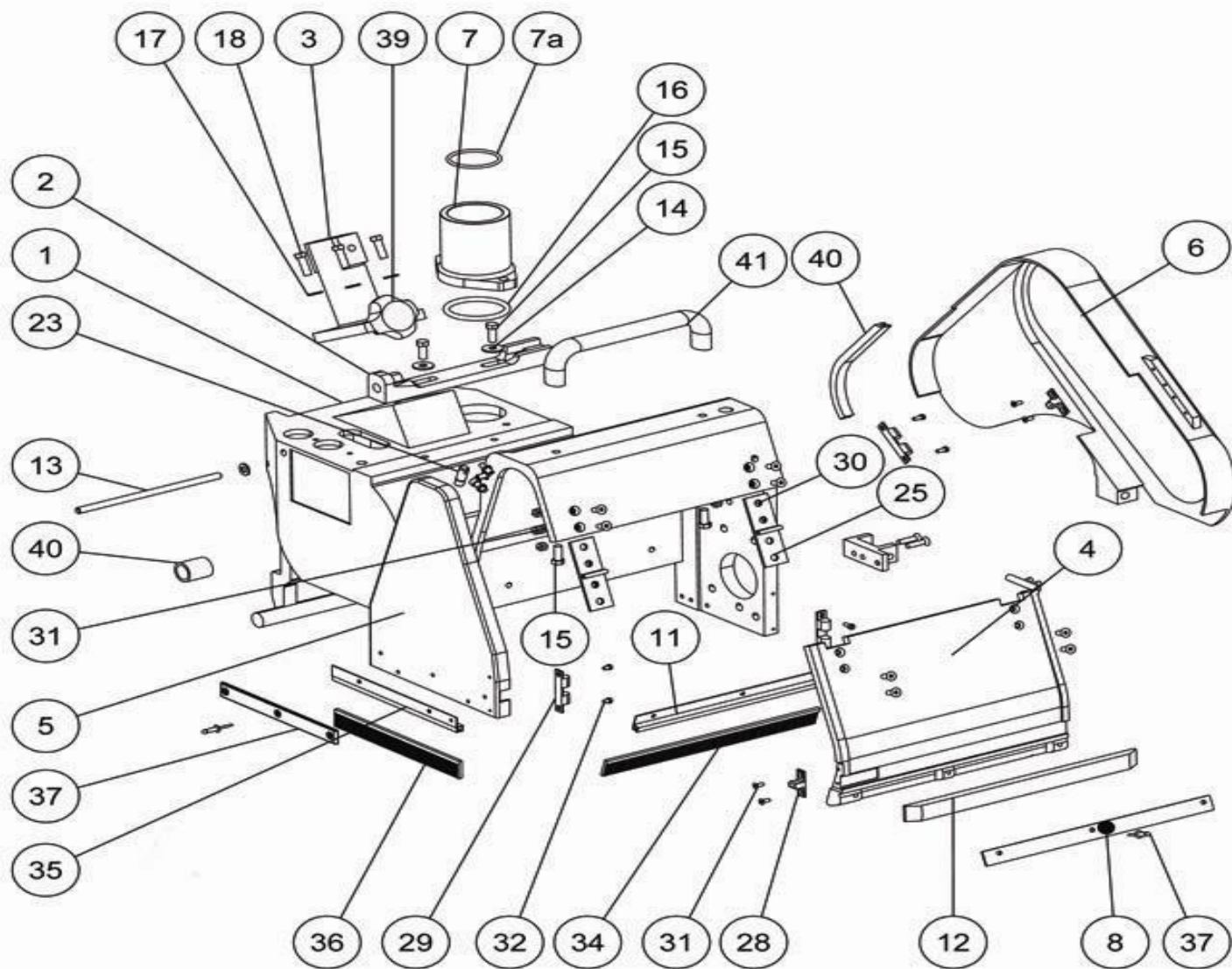
Bona Belt Previous Models AMO110020.3 Belt chassis A
