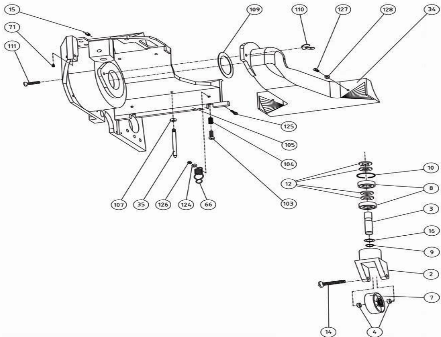
Bona Belt Previous Models AMO110020.3 Belt rear wheel
