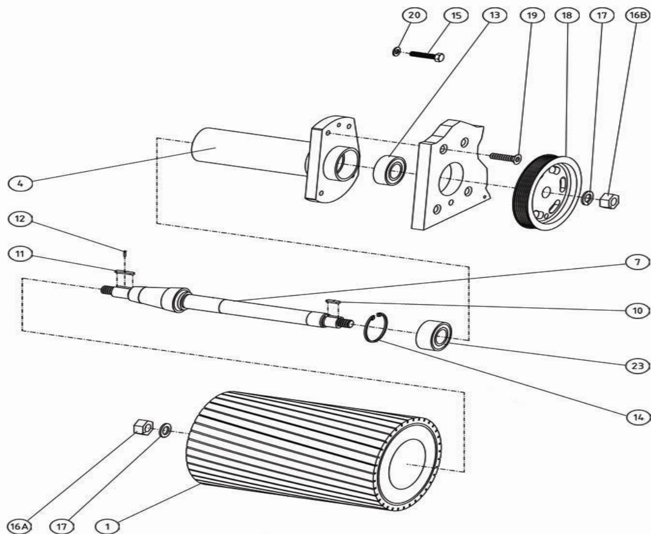
Bona Belt Previous Models AMO110020.3 Belt sanding drum
