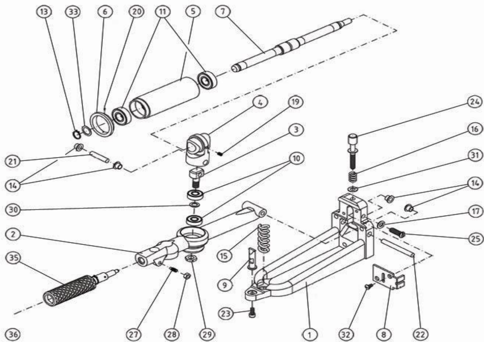
Bona Belt Previous Models AMO110020.3 Belt Tension device
