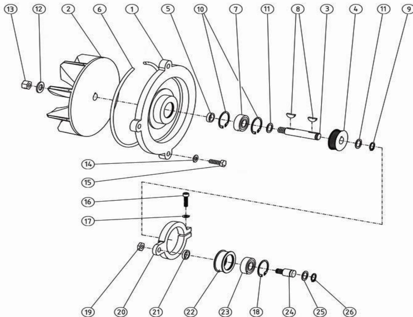
Bona Belt Previous Models AMO110020.3 Belt vacuum cleaner
