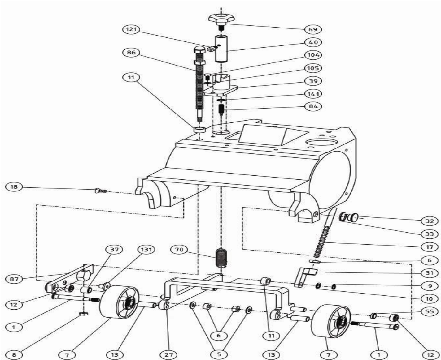
Bona Belt Previous Models AMO110020.3 Belt wheel subframe
