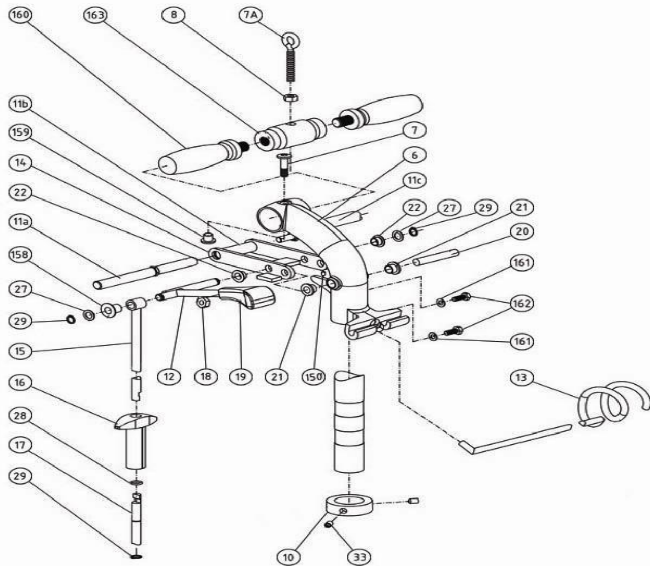
Bona Flexidrum Previous Models AMO150009.1 Flexidrum main handle
