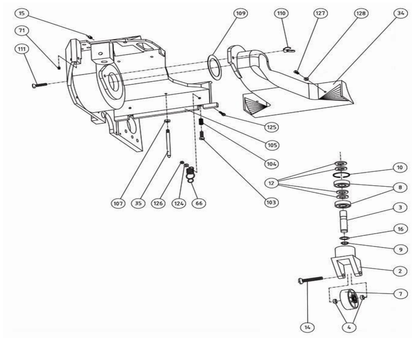
Bona Flexidrum Previous Models AMO150009.1 Flexidrum rear wheel/intake duct complete
