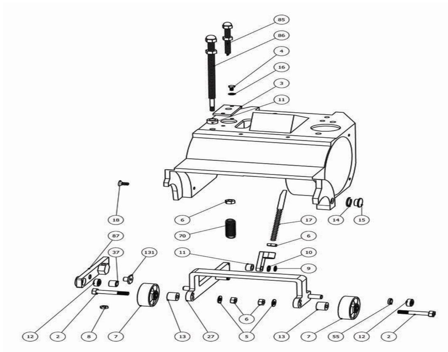
Bona Flexidrum Previous Models AMO150009.1 Flexidrum wheel subframe
