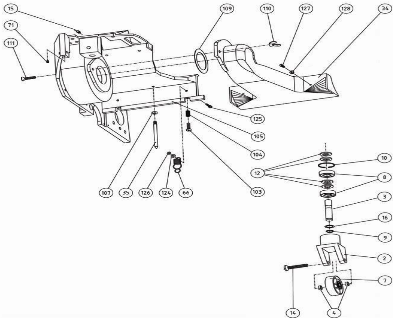
Bona Belt Previous Models AM0003150 Belt Rear Wheel
