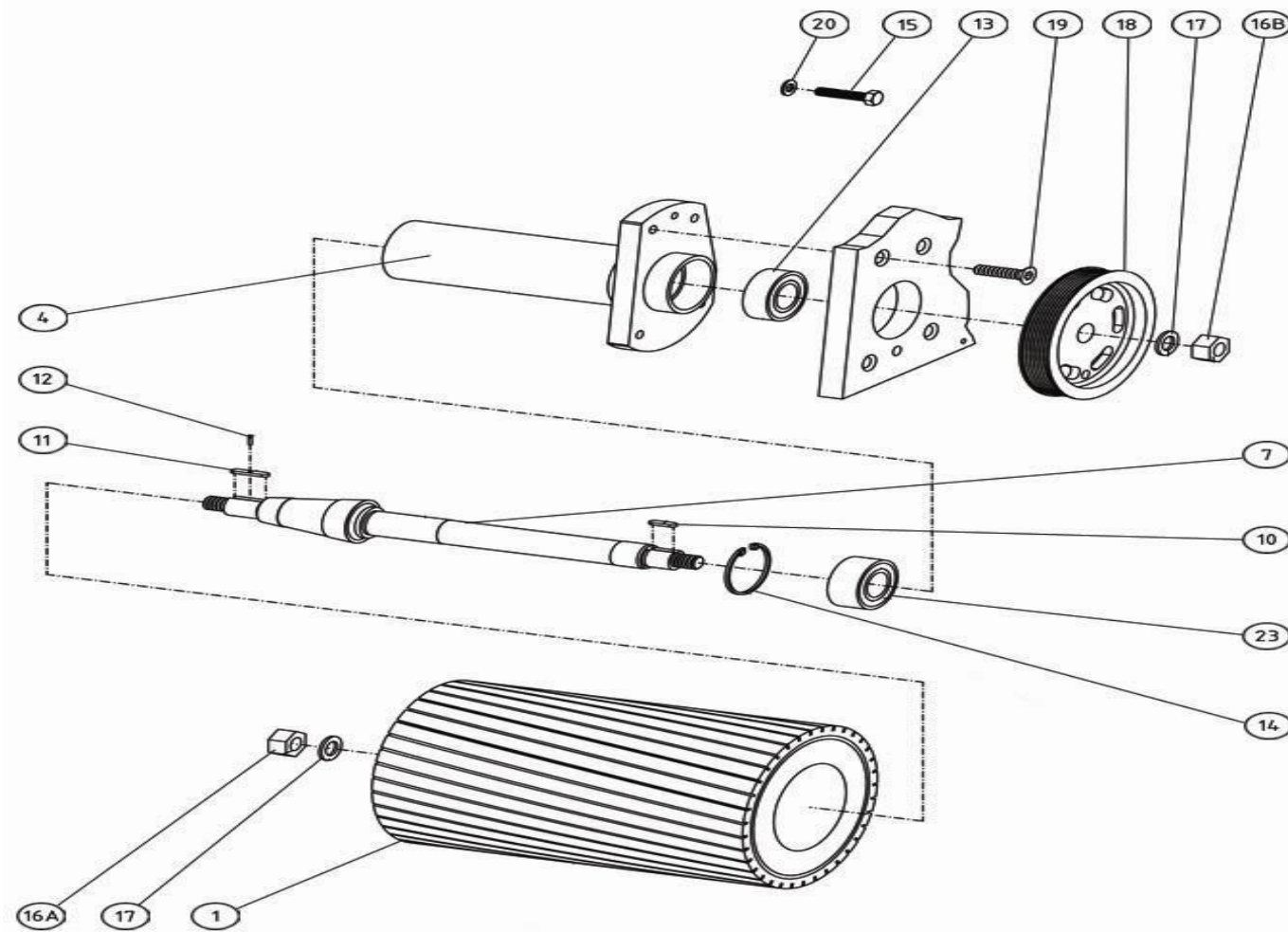
Bona Belt Previous Models AM0003150 Belt Sanding drum
