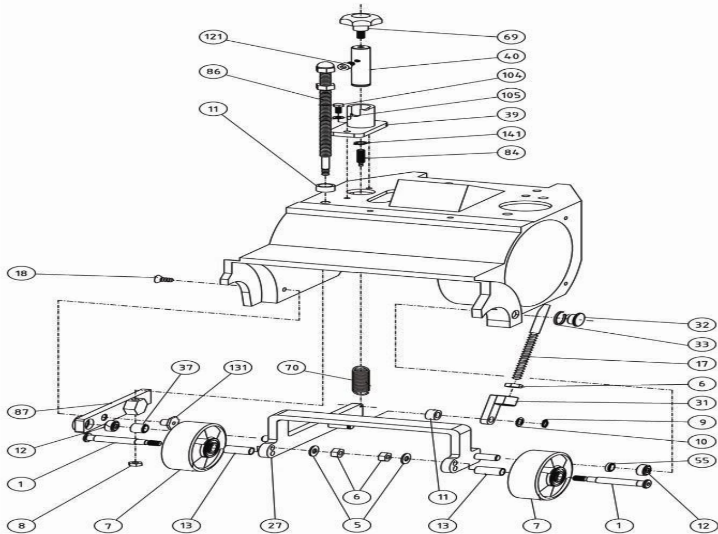
Bona Belt Previous Models AM0003150 Belt Wheel Subframe
