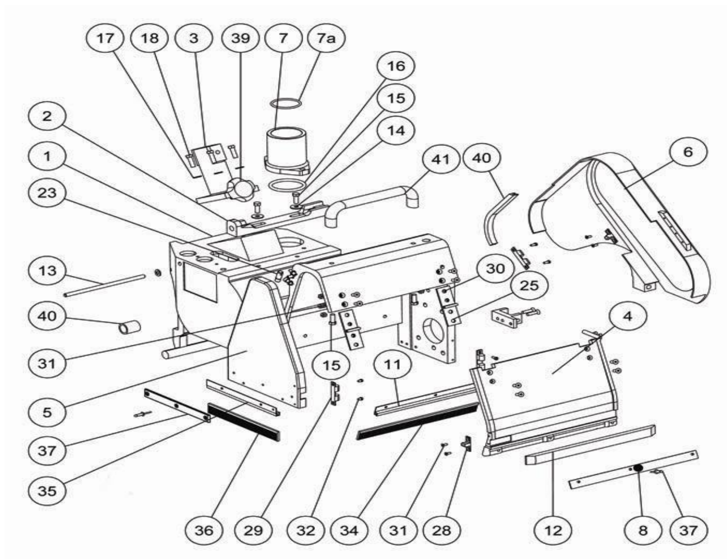
Bona Belt Previous Models AMO110015.3 Belt chassis A
