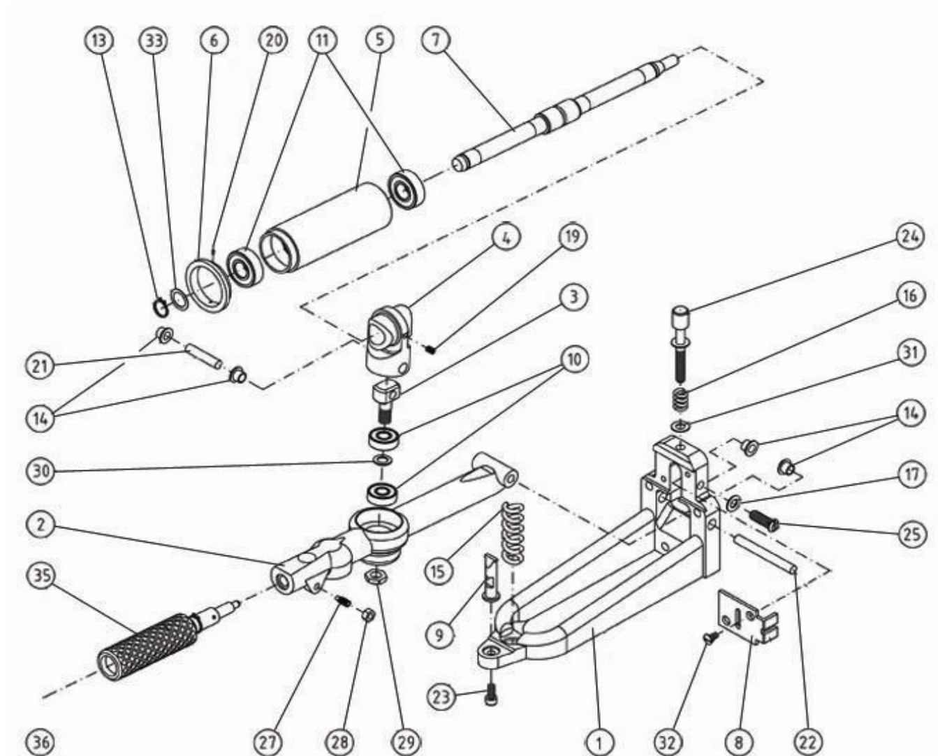
Bona Belt Previous Models AMO110015.3 Belt Tension device
