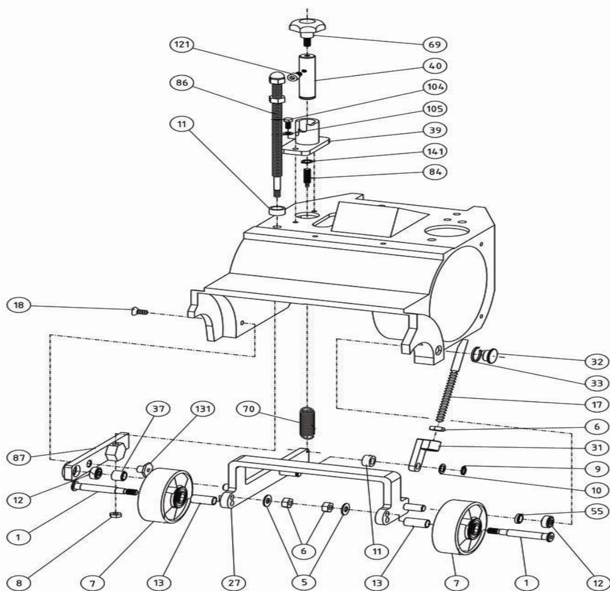
Bona Belt Previous Models AMO110015.3 Belt wheel subframe
