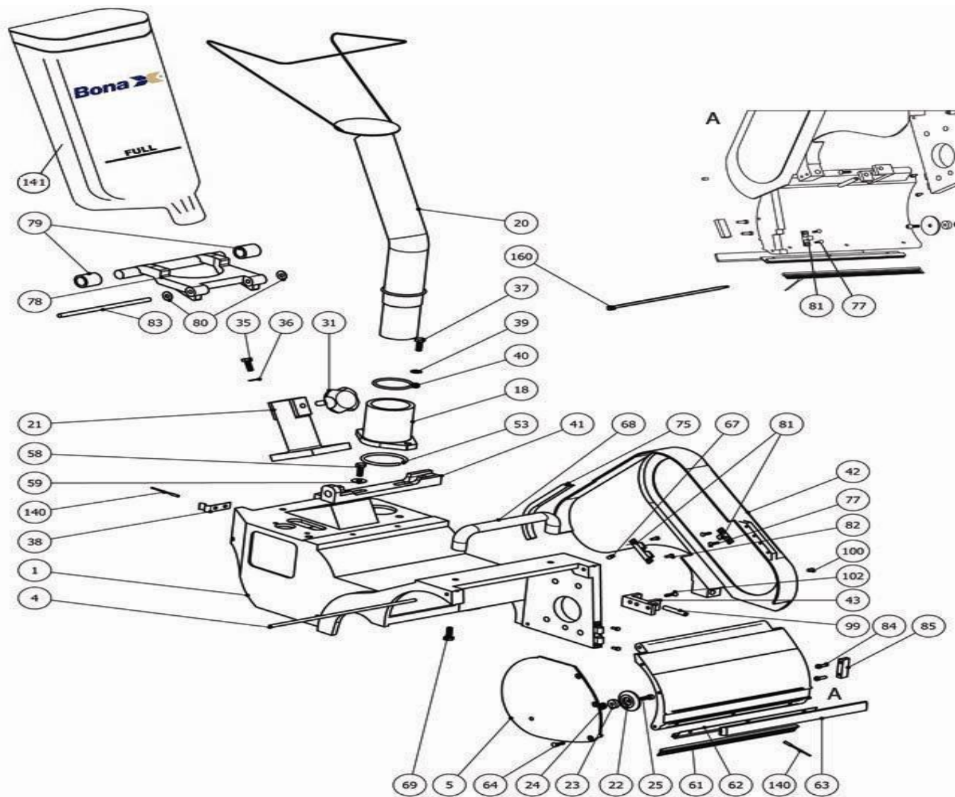
Bona Flexidrum Previous Models AMO150006.2 Flexidrum housing
