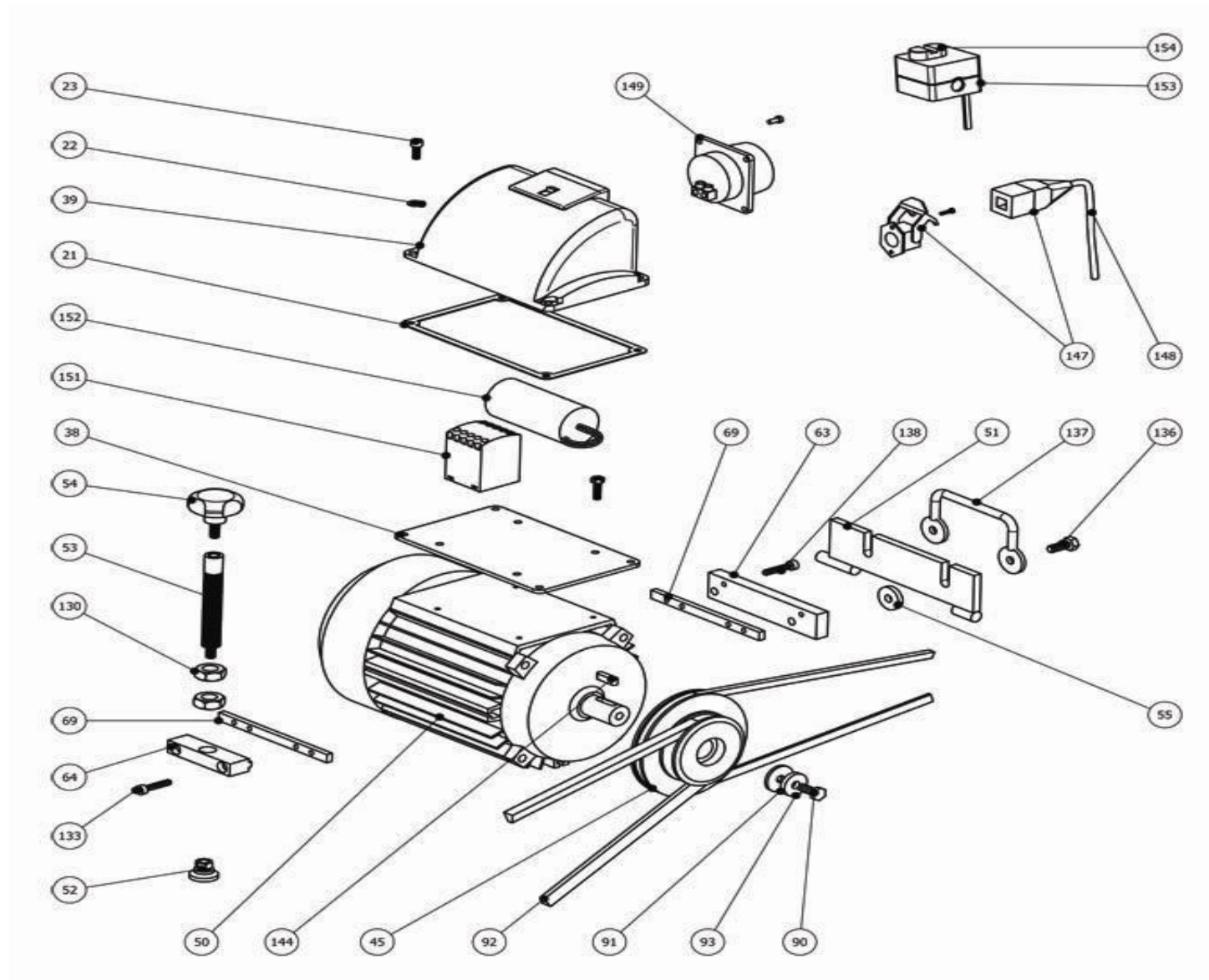
Bona Flexidrum Previous Models AMO150006.2 Flexidrum Motor 1,8KW
