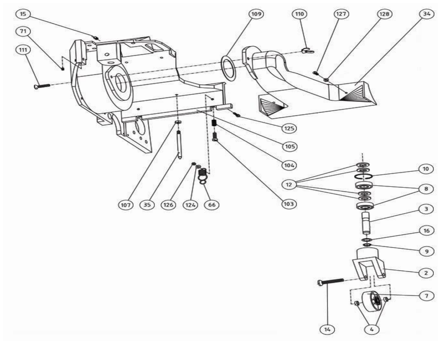
Bona Flexidrum Previous Models AMO150006.2 Flexidrum rear wheel
