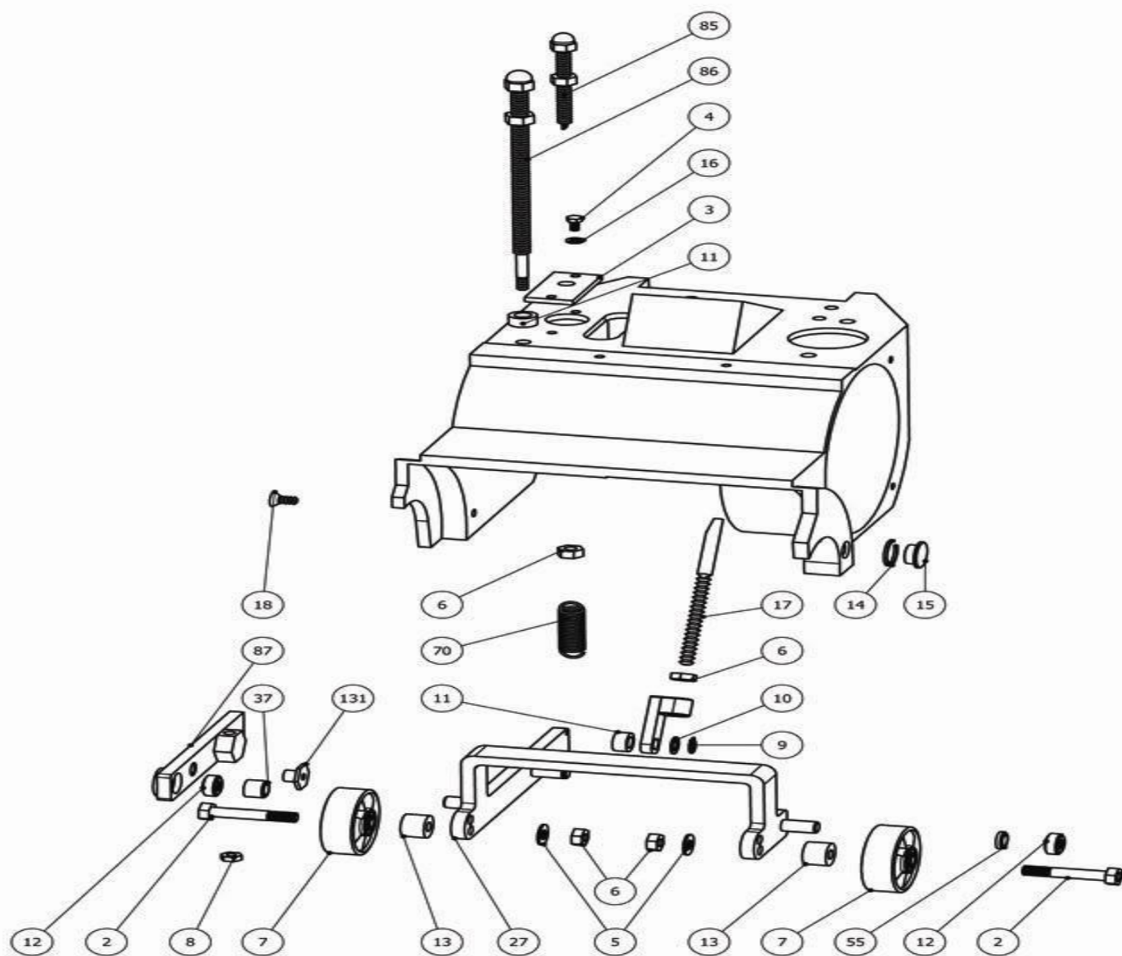
Bona Flexidrum Previous Models AMO150006.2 Flexidrum wheel subframe
