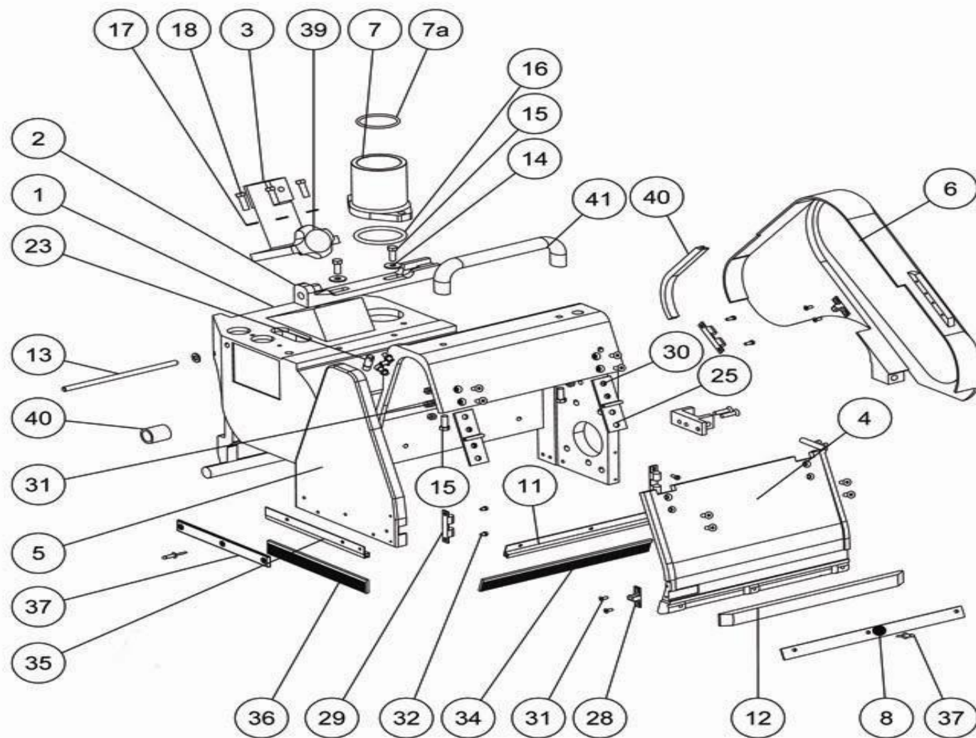
Bona Belt Previous Models AMO110013.3 Belt chassis A
