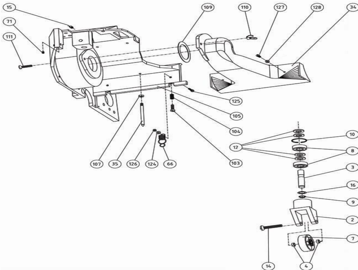
Bona Belt Previous Models AMO110013.3 Belt rear wheel
