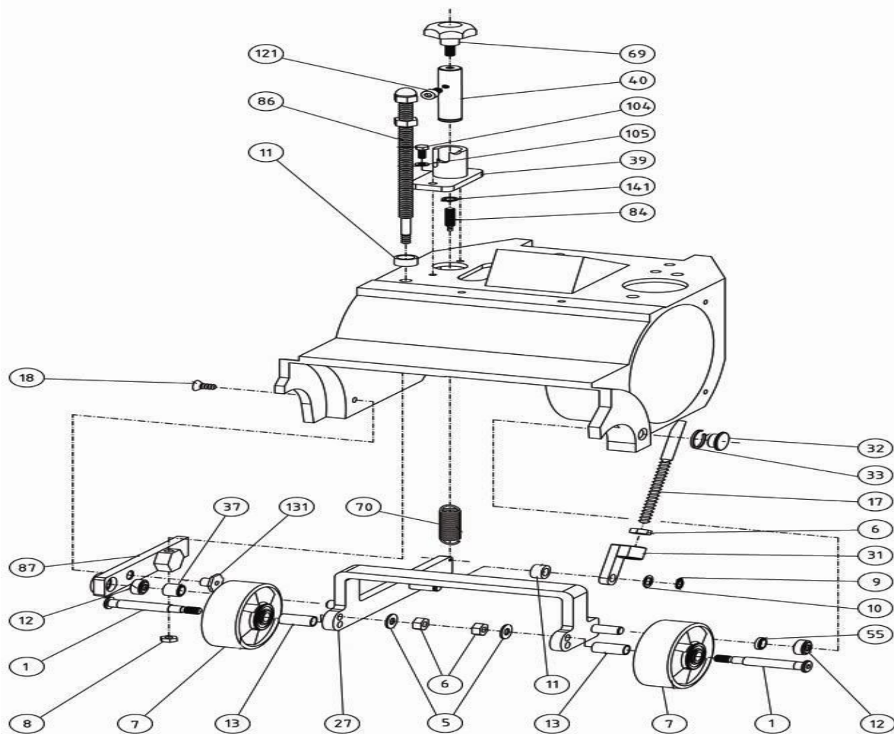
Bona Belt Previous Models AMO110013.3 Belt wheel subframe
