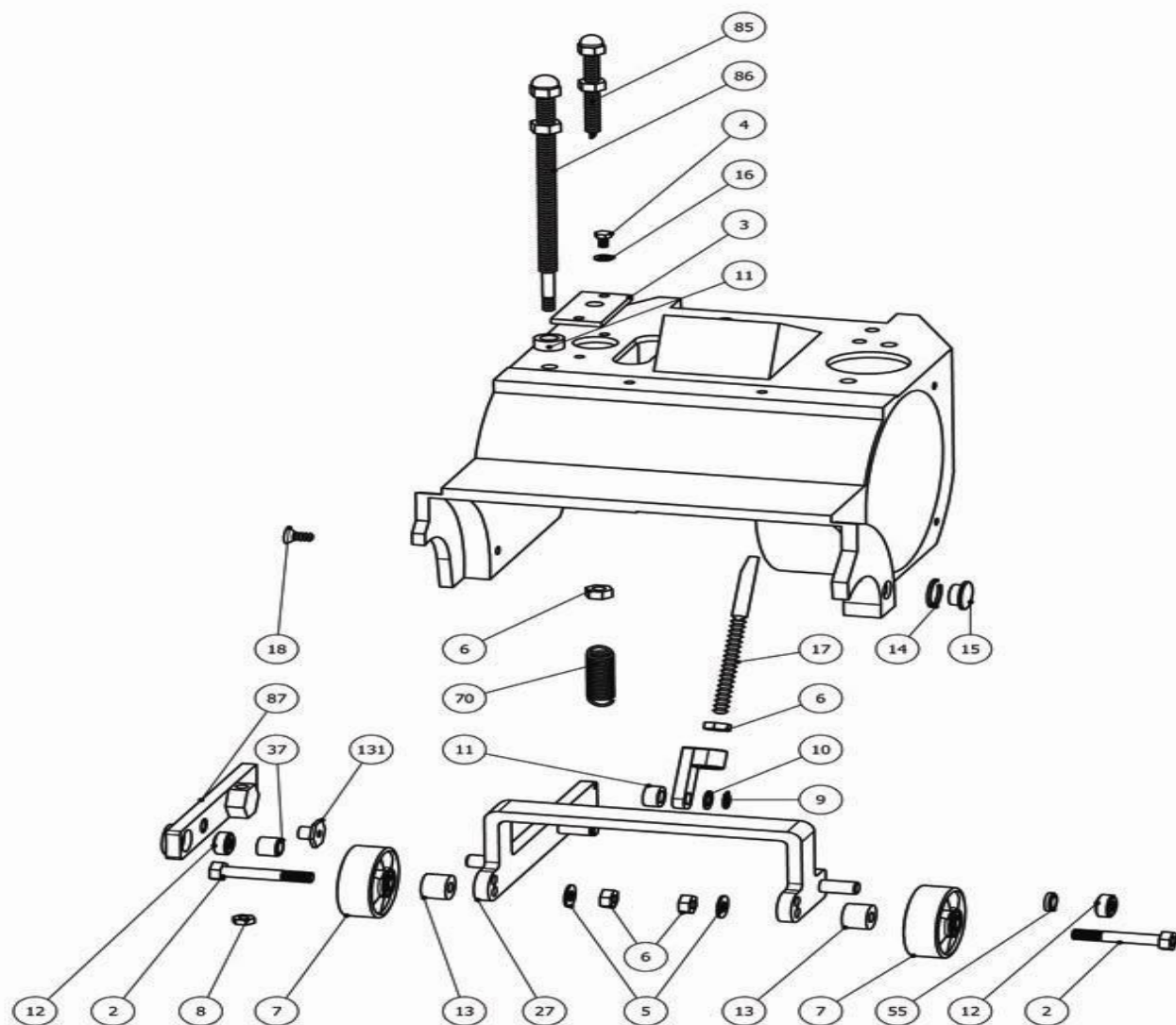
Bona Flexidrum Previous Models AMO150000.1 Flexidrum wheel subframe
