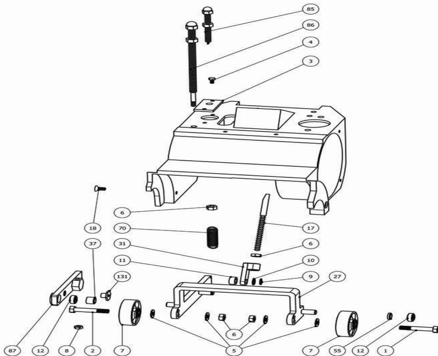
Bona Midi AMO150003.0 Midi wheel subframe
