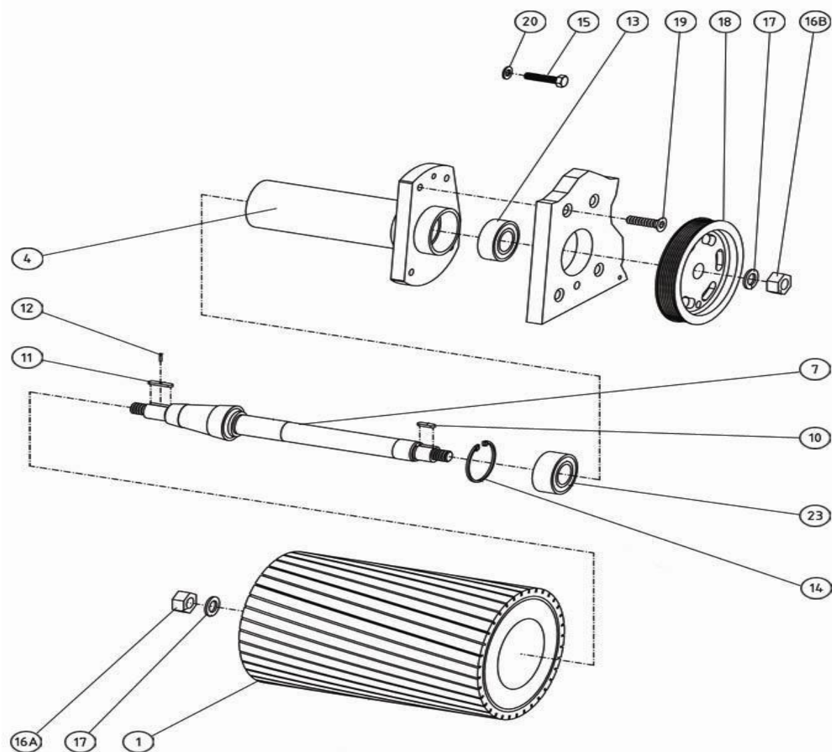
Bona Belt Previous Models AMO110025.3 Belt sanding drum
