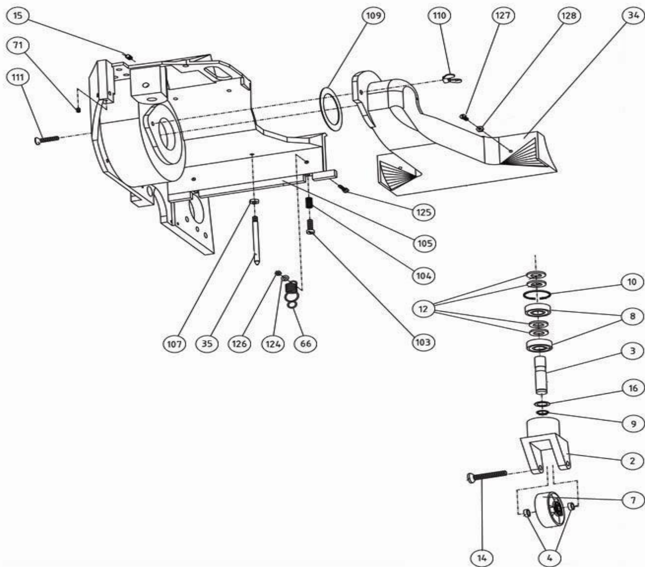
Bona Belt Previous Models AMO110025.3 Belt Wheel subframe
