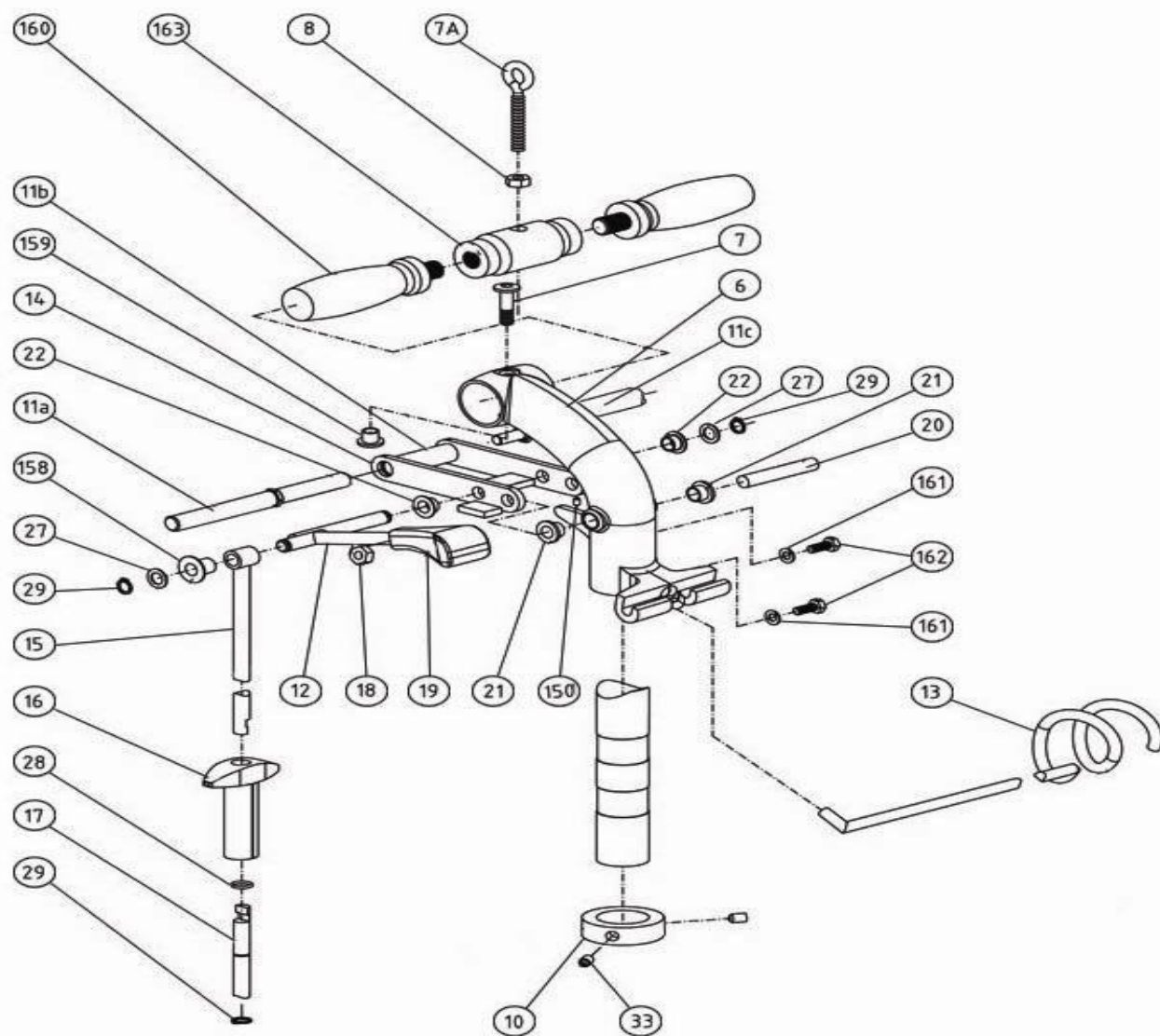
Bona Flexidrum Previous Models AMO150004.3 Flexidrum handle
