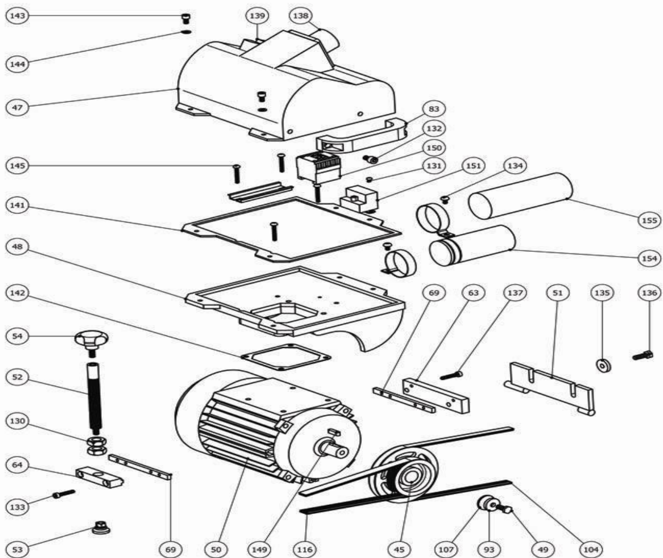
Bona Flexidrum Previous Models AMO150004.3 Flexidrum Motor 2,2KW
