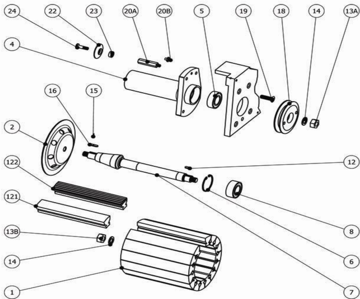
Bona Flexidrum Previous Models AMO150004.3 Flexidrum sanding drum
