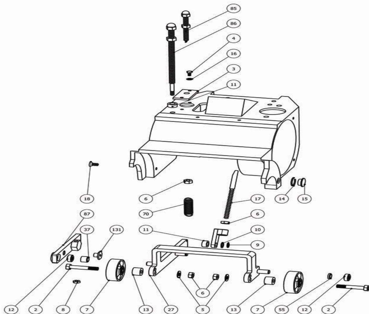
Bona Flexidrum Previous Models AMO150004.3 Flexidrum wheel subframe
